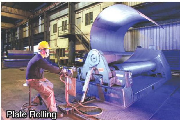
Plate Bending
